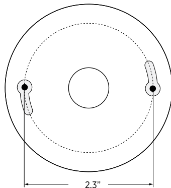
Bottom of Camera (Mounting Holes)
